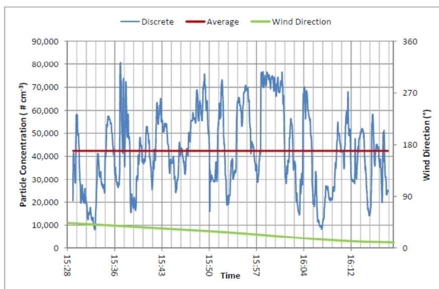
Fig 19: Terminal 5 – entire sampling period
