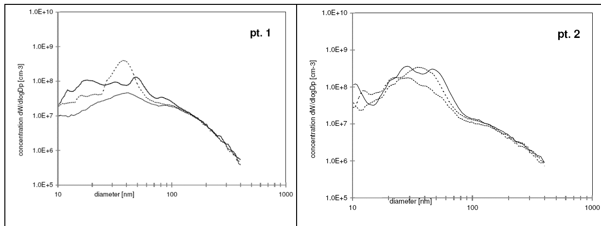
Fig 15: Particle size-number concentration distribution of a 2004 Deutz 139kW Ground Power Unit (pt.1 = 30% dummy load, pt. 2 = 60% dummy load); 3 samples each with NanoMet-diluter at exhaust pipe
