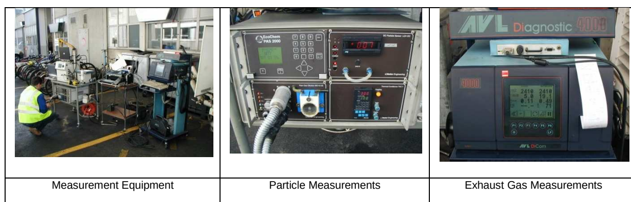
Fig 14: Measurement equipment for GPU measurements
