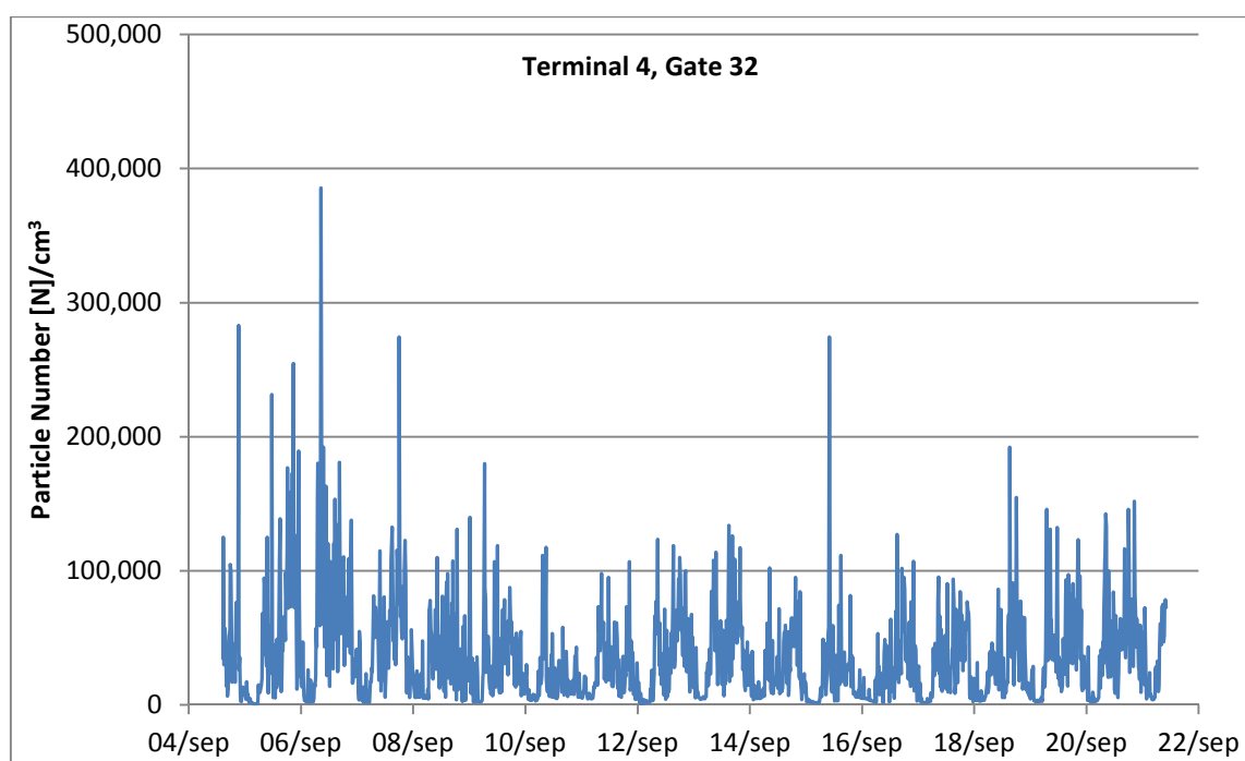
Fig 23: Terminal 4 – Number of ultrafine particles (size range from 0,004 \mu\text{m} ) 15 minutes average
