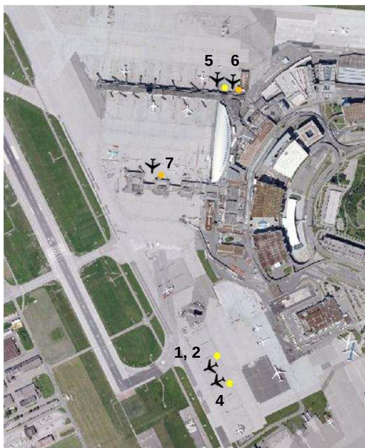
Fig 16: Measurement points and locations Zurich airport (MP1-7) (yellow: July 2012, orange: August 2012)
