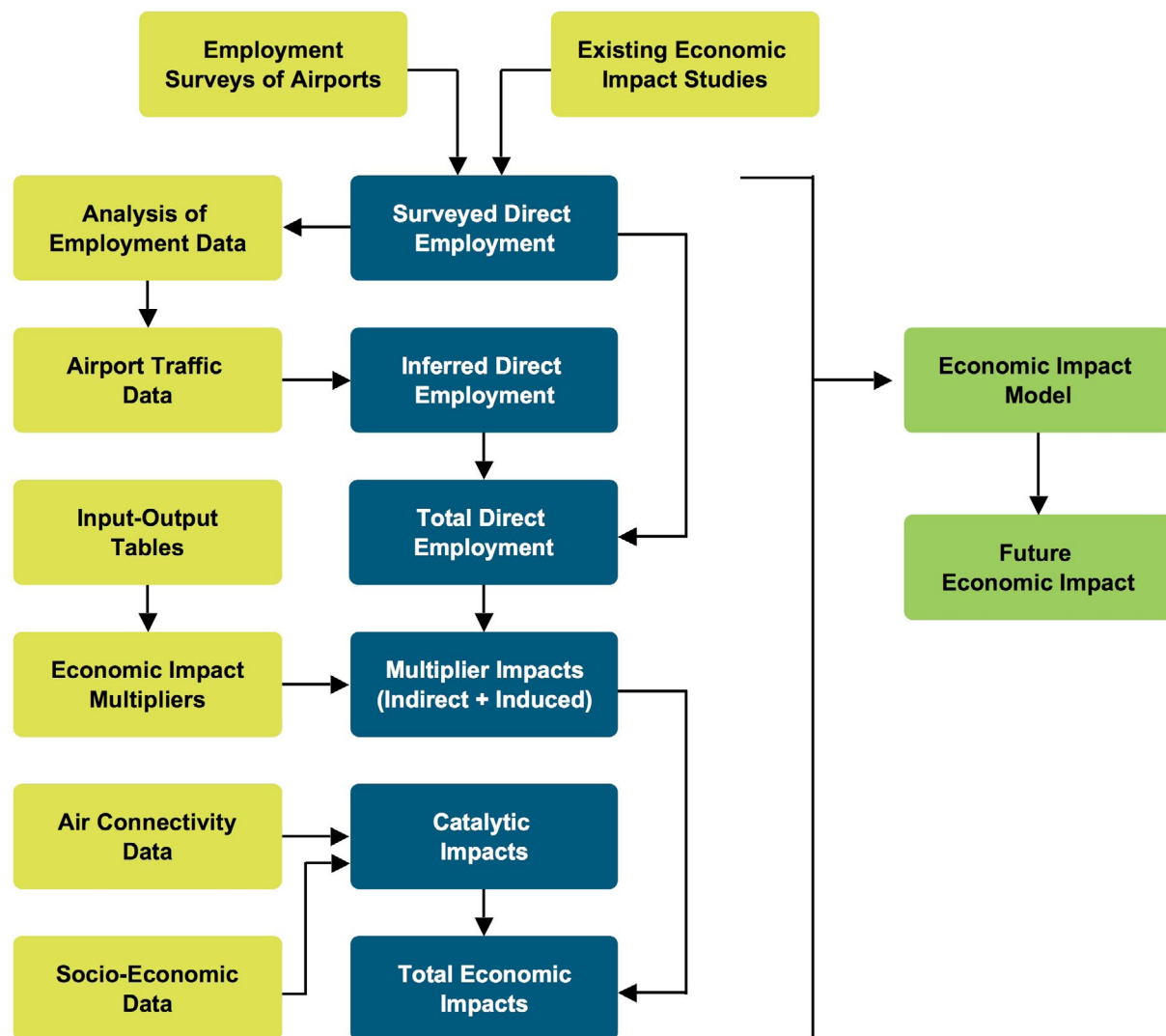
Figure 4-1: Study Methodology
